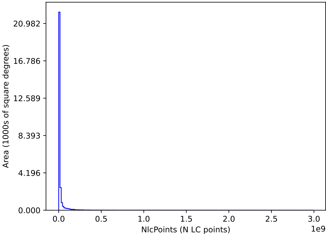
too_elab_r256_d3_ugrizy_v3.4_10yrs : NlcPoints
