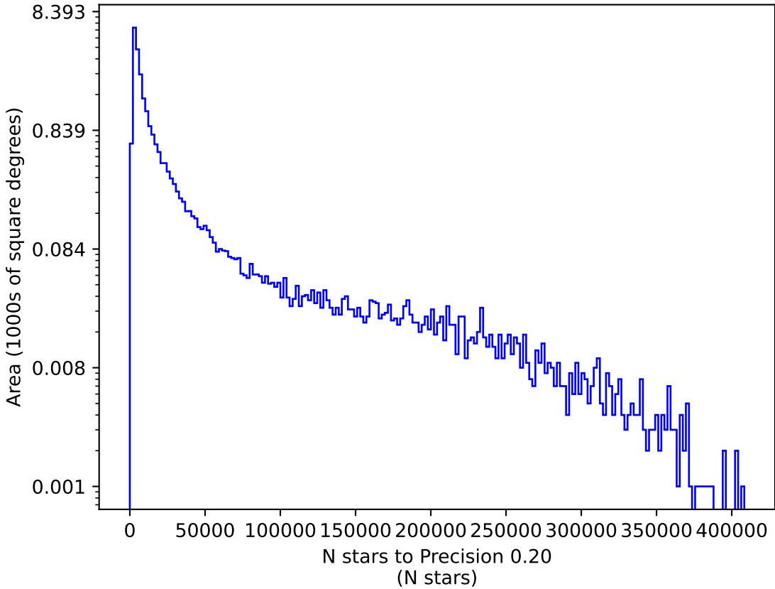
too_elab_r256_d3_ugrizy_v3.4_10yrs u: N stars to Precision 0.20
