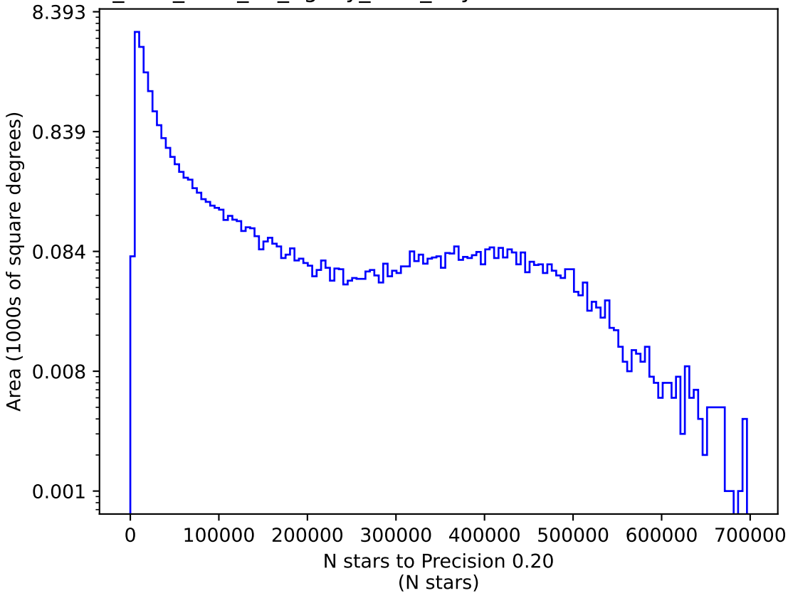
too_elab_r256_d3_ugrizy_v3.4_10yrs i: N stars to Precision 0.20
