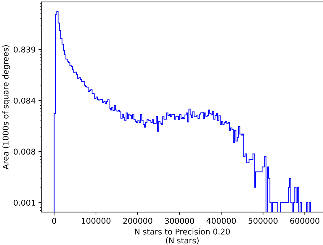
too_elab_r256_d3_ugrizy_v3.4_10yrs g: N stars to Precision 0.20
