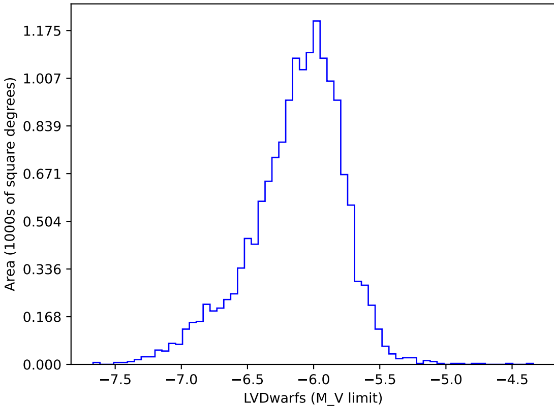
too_elab_r256_d3_ugrizy_v3.4_10yrs gi: LVDwarfs
