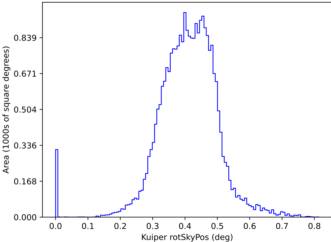
too_elab_r256_d3_ugrizy_v3.4_10yrs y: Kuiper rotSkyPos
