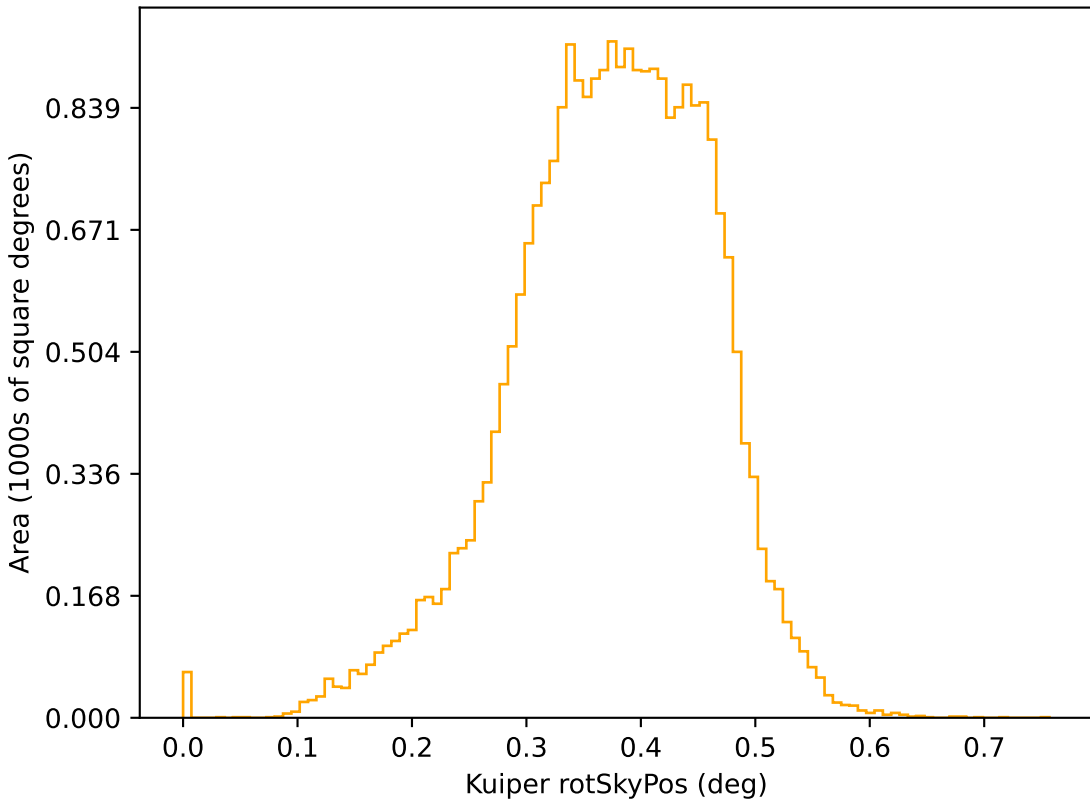
too_elab_r256_d3_ugrizy_v3.4_10yrs r: Kuiper rotSkyPos
