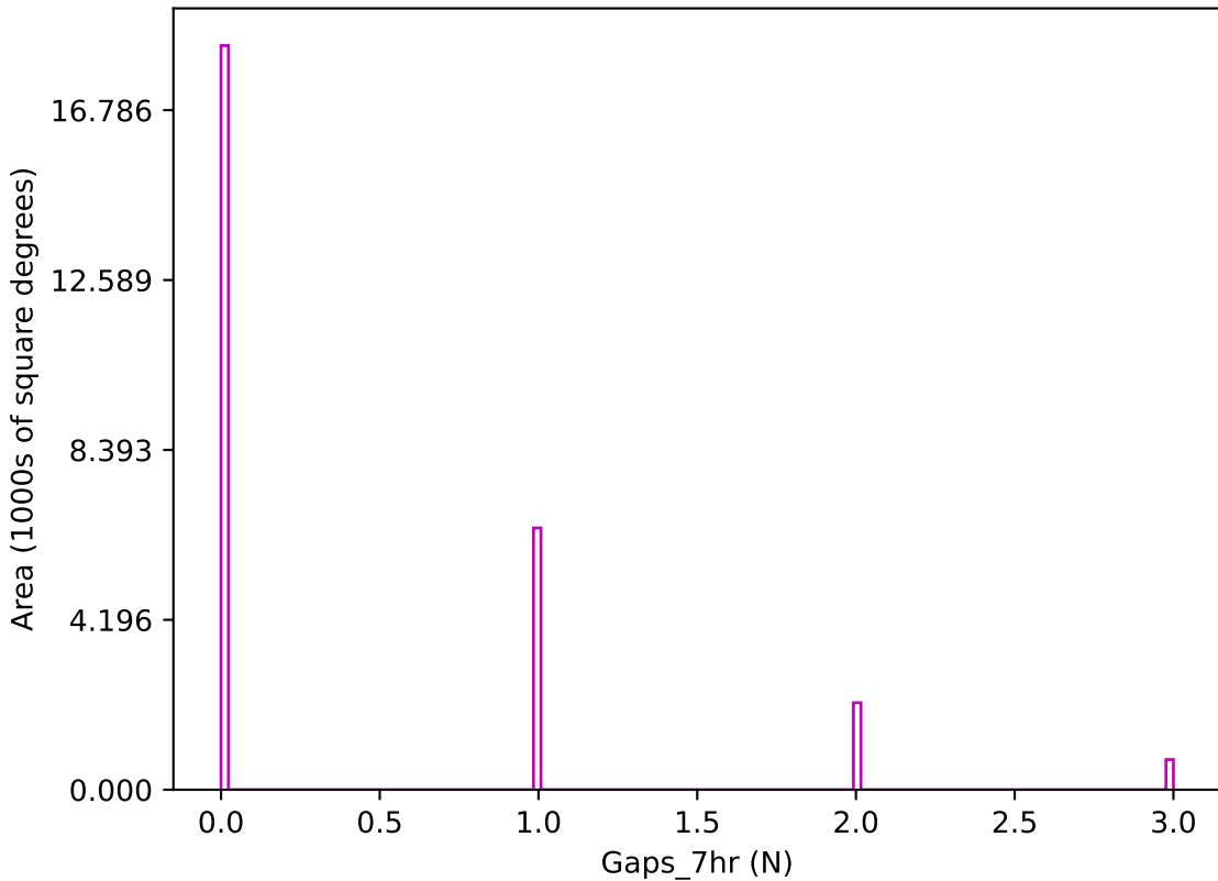
too_elab_r256_d3_ugrizy_v3.4_10yrs z band: Gaps_7hr
