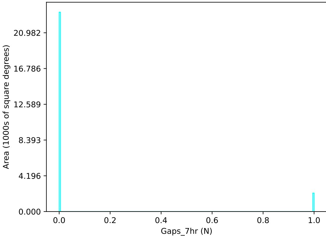
too_elab_r256_d3_ugrizy_v3.4_10yrs u band: Gaps_7hr
