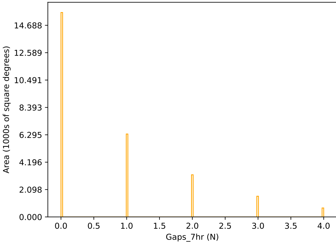
too_elab_r256_d3_ugrizy_v3.4_10yrs r band: Gaps_7hr
