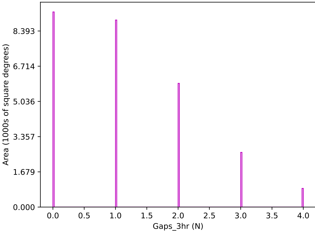
too_elab_r256_d3_ugrizy_v3.4_10yrs z band: Gaps_3hr
