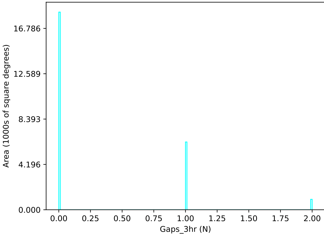
too_elab_r256_d3_ugrizy_v3.4_10yrs u band: Gaps_3hr
