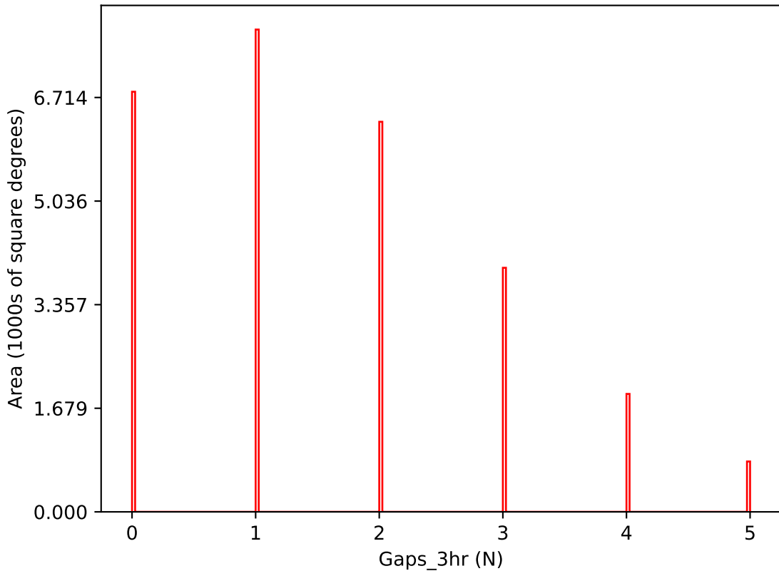
too_elab_r256_d3_ugrizy_v3.4_10yrs i band: Gaps_3hr
