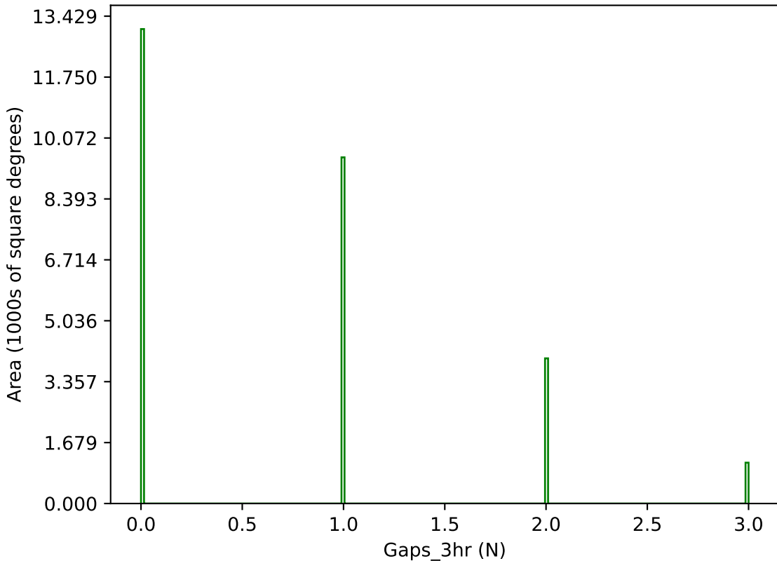
too_elab_r256_d3_ugrizy_v3.4_10yrs g band: Gaps_3hr
