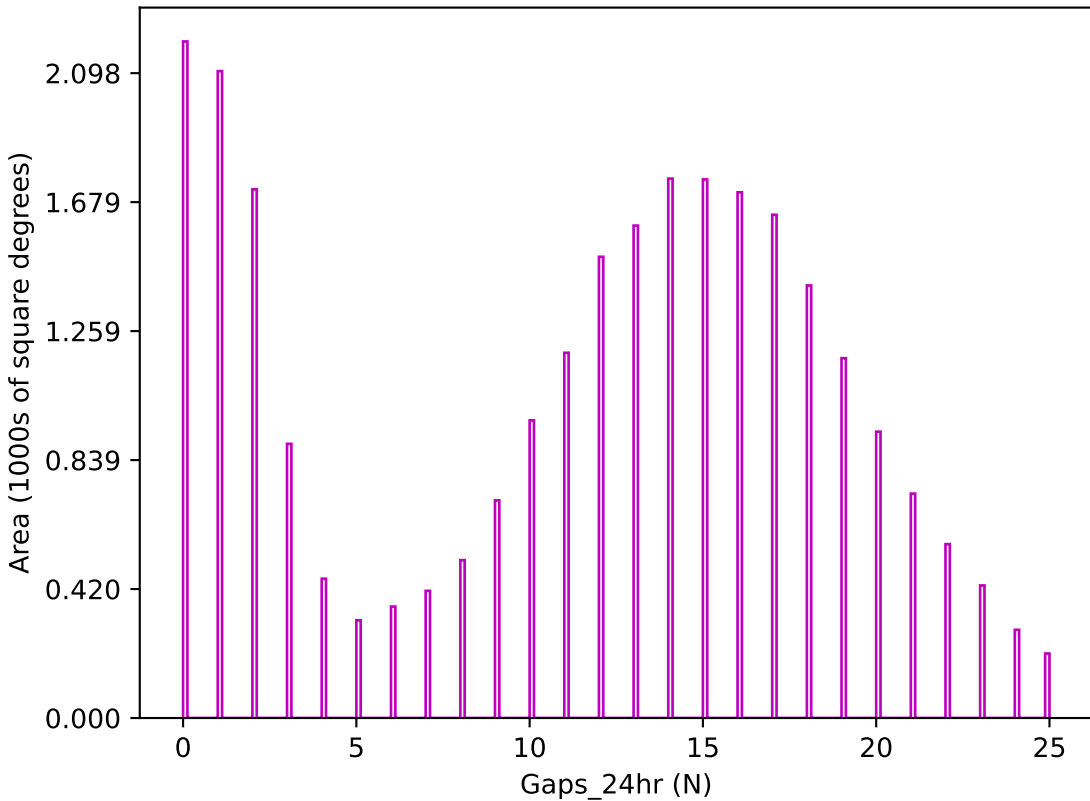
too_elab_r256_d3_ugrizy_v3.4_10yrs z band: Gaps_24hr
