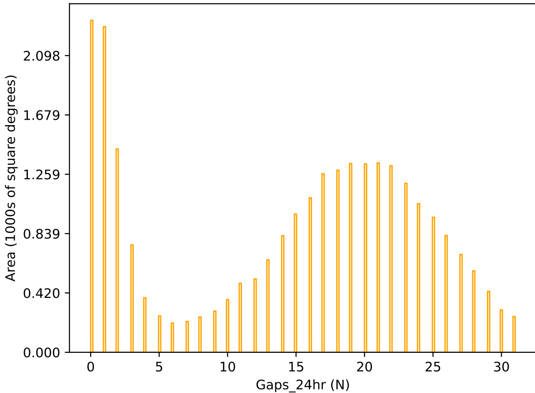
too_elab_r256_d3_ugrizy_v3.4_10yrs r band: Gaps_24hr
