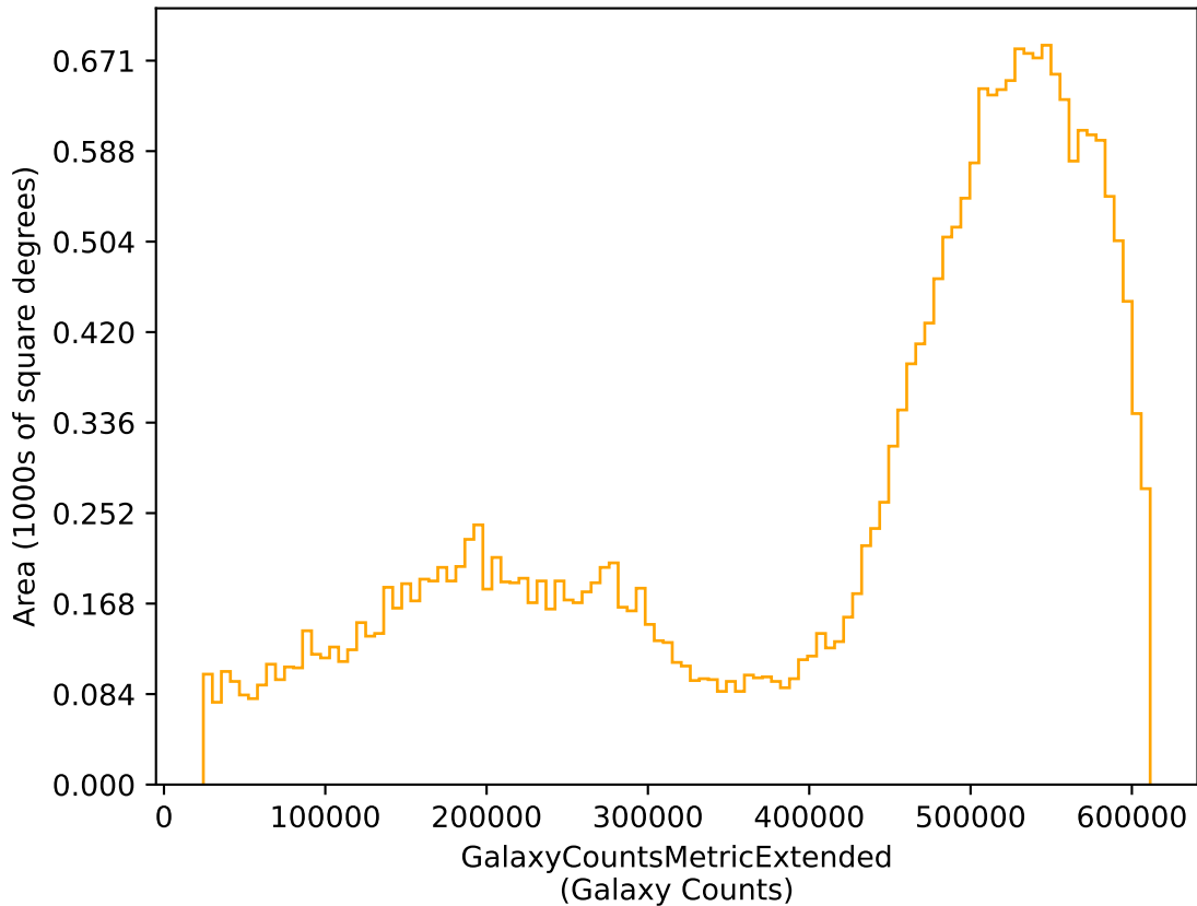
too_elab_r256_d3_ugrizy_v3.4_10yrs r: GalaxyCountsMetricExtended
