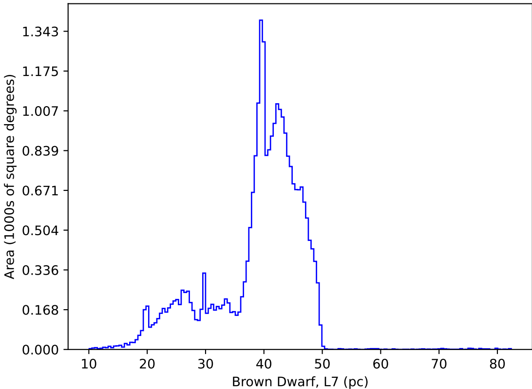
too_elab_r256_d3_ugrizy_v3.4_10yrs : Brown Dwarf, L7
