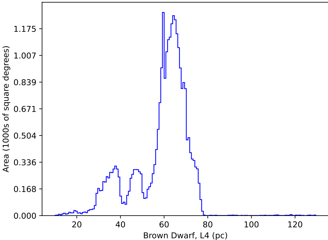
too_elab_r256_d3_ugrizy_v3.4_10yrs : Brown Dwarf, L4
