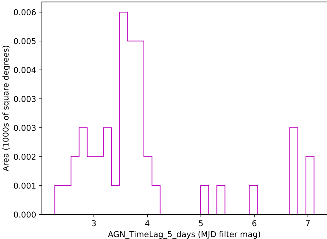
too_elab_r256_d3_ugrizy_v3.4_10yrs z band: AGN_TimeLag_5_days
