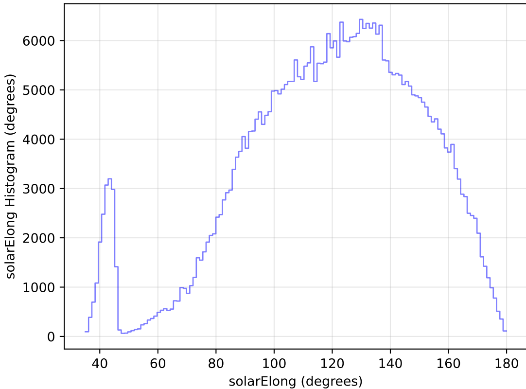
too_elab_r256_d3_ugrizy_v3.4_10yrs WFD z band: solarElong Histogram
