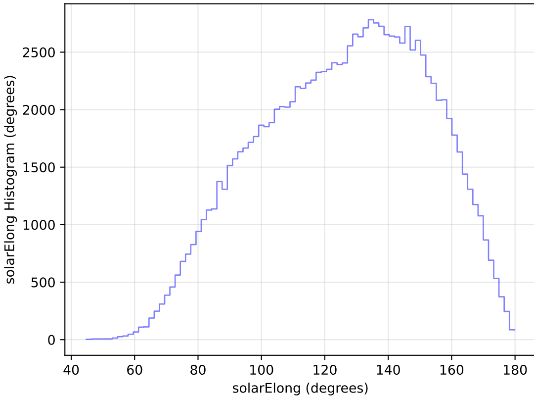
too_elab_r256_d3_ugrizy_v3.4_10yrs WFD u band: solarElong Histogram
