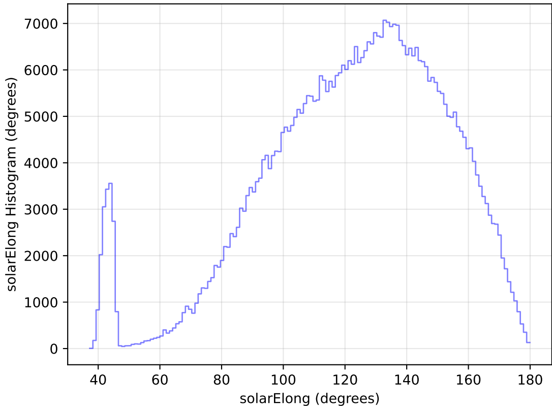
too_elab_r256_d3_ugrizy_v3.4_10yrs WFD r band: solarElong Histogram
