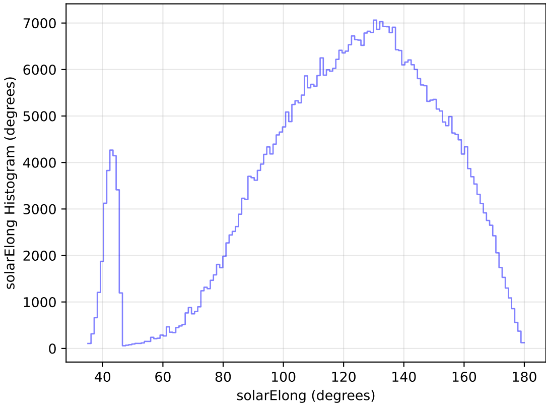
too_elab_r256_d3_ugrizy_v3.4_10yrs WFD i band: solarElong Histogram
