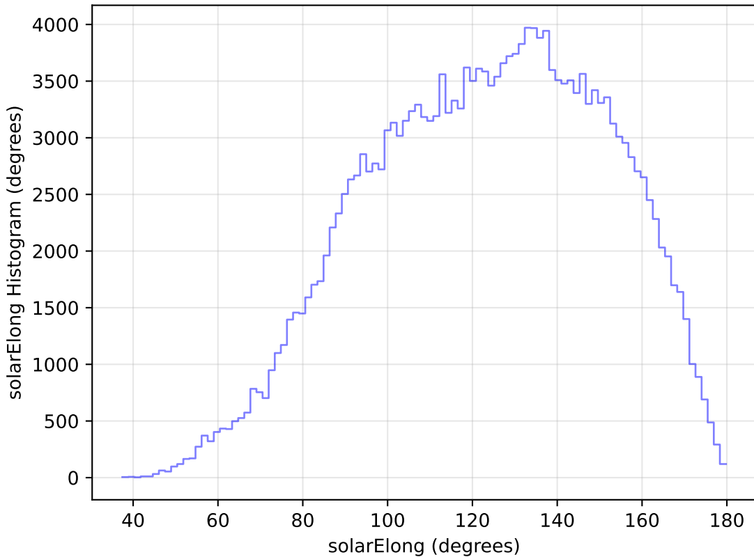
too_elab_r256_d3_ugrizy_v3.4_10yrs WFD g band: solarElong Histogram
