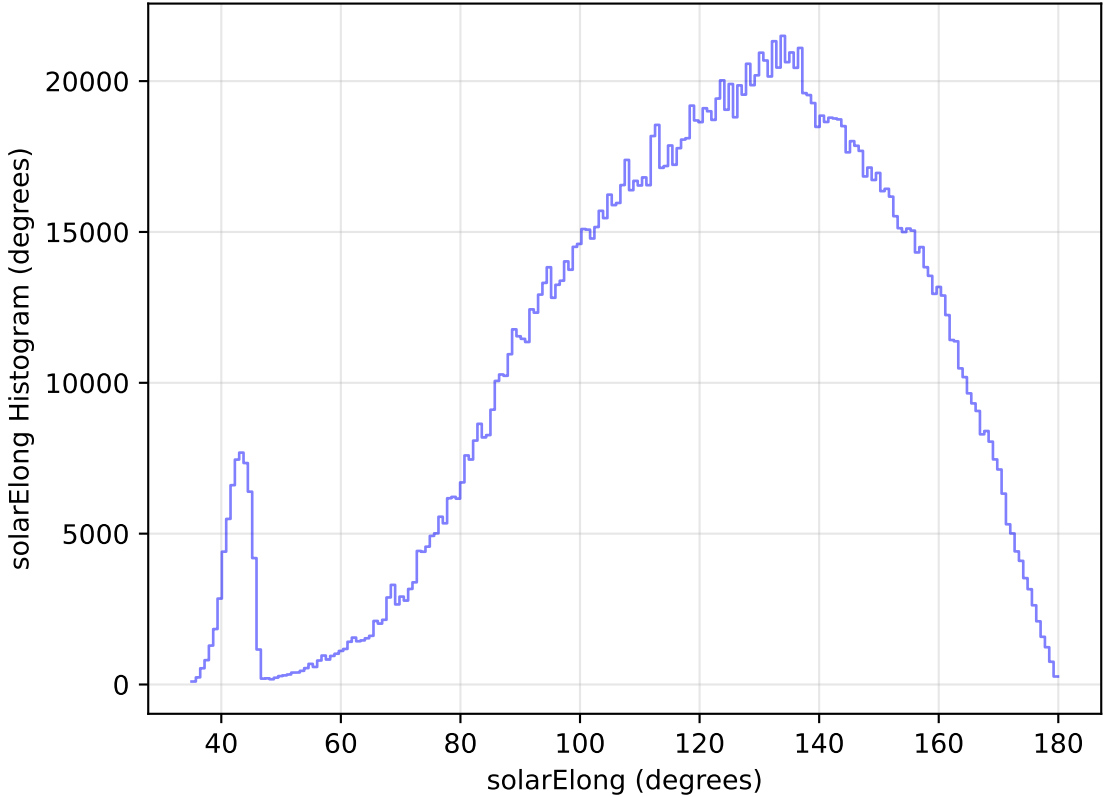
too_elab_r256_d3_ugrizy_v3.4_10yrs WFD all bands: solarElong Histogram
