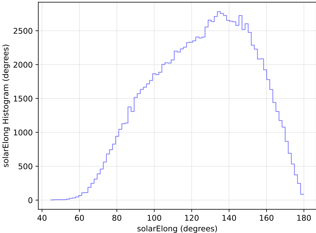
too_elab_r256_d3_ugrizy_v3.4_10yrs All sky u band: solarElong Histogram
