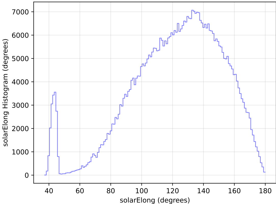
too_elab_r256_d3_ugrizy_v3.4_10yrs All sky r band: solarElong Histogram
