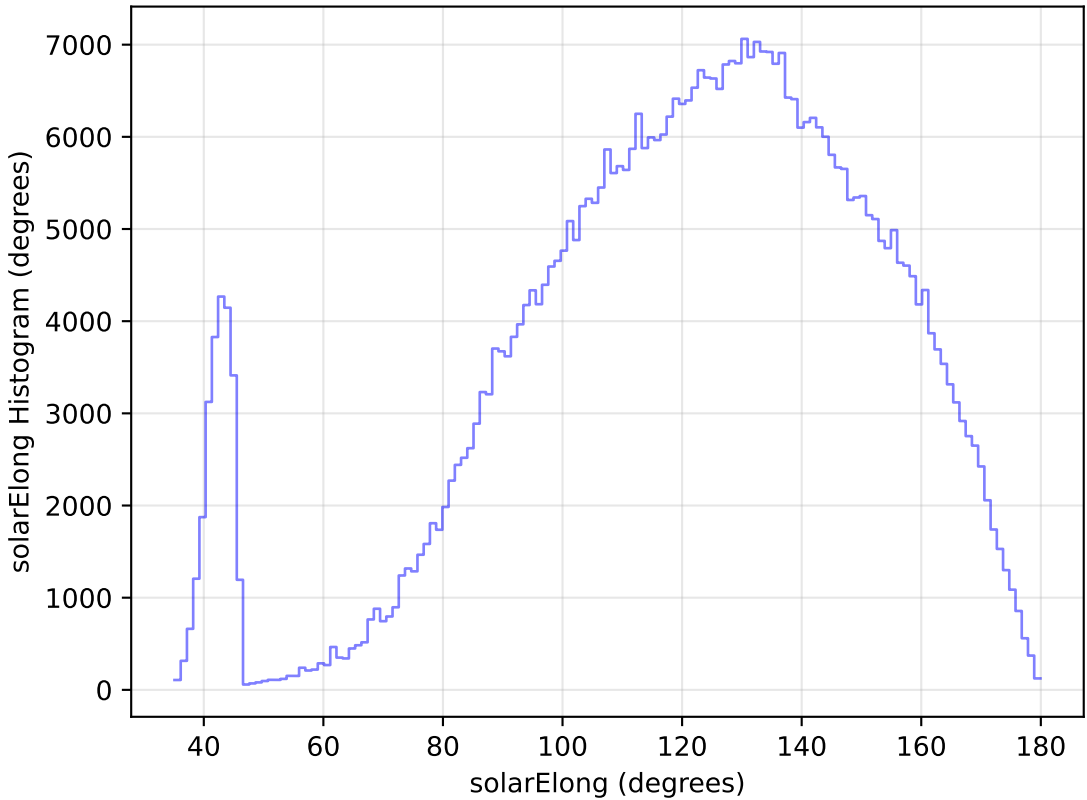
too_elab_r256_d3_ugrizy_v3.4_10yrs All sky i band: solarElong Histogram
