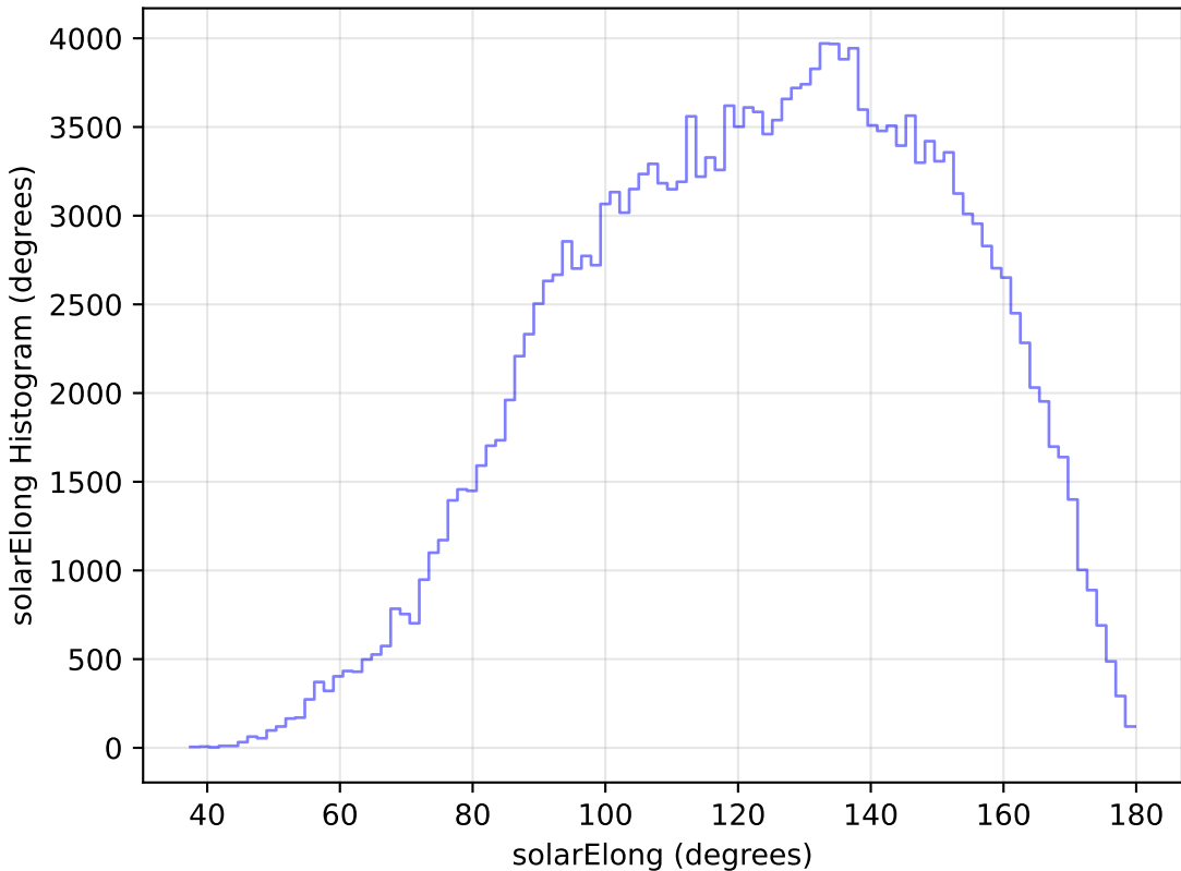
too_elab_r256_d3_ugrizy_v3.4_10yrs All sky g band: solarElong Histogram
