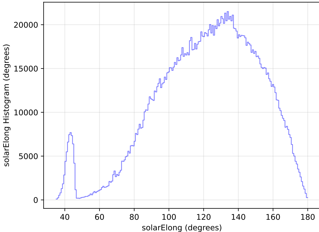
too_elab_r256_d3_ugrizy_v3.4_10yrs All sky all bands: solarElong Histogram
