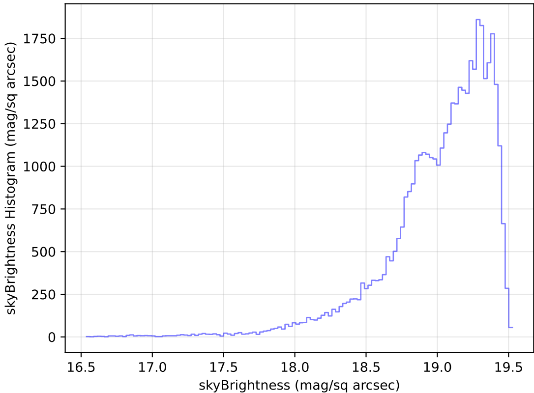
too_elab_r256_d3_ugrizy_v3.4_10yrs Yr 1 z band: skyBrightness Histogram
