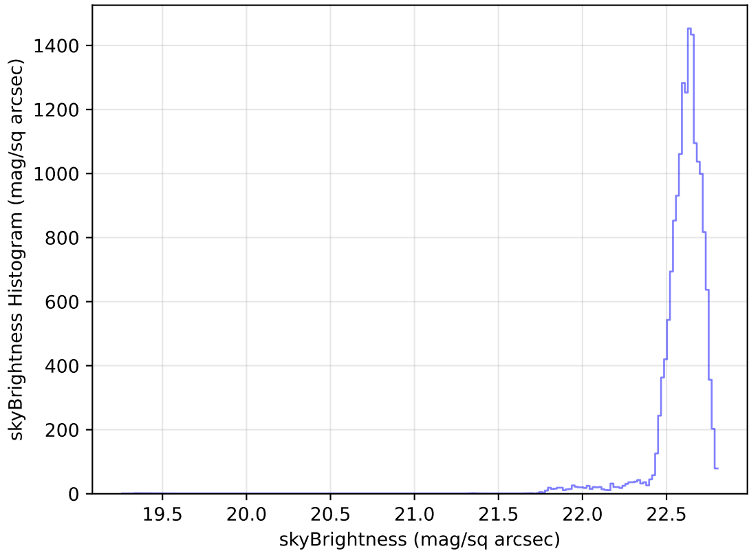
too_elab_r256_d3_ugrizy_v3.4_10yrs Yr 1 u band: skyBrightness Histogram
