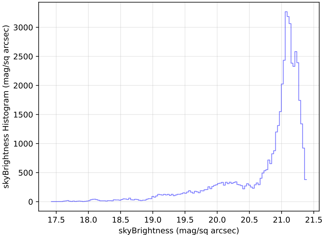
too_elab_r256_d3_ugrizy_v3.4_10yrs Yr 1 r band: skyBrightness Histogram
