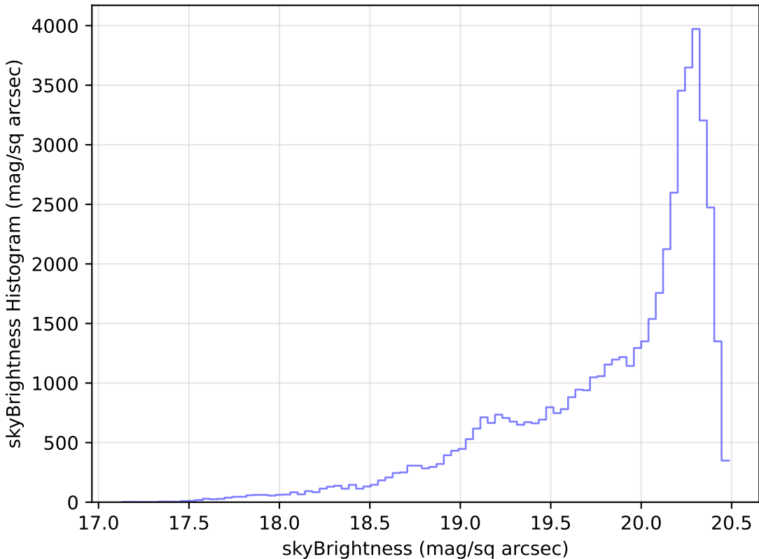
too_elab_r256_d3_ugrizy_v3.4_10yrs Yr 1 i band: skyBrightness Histogram
