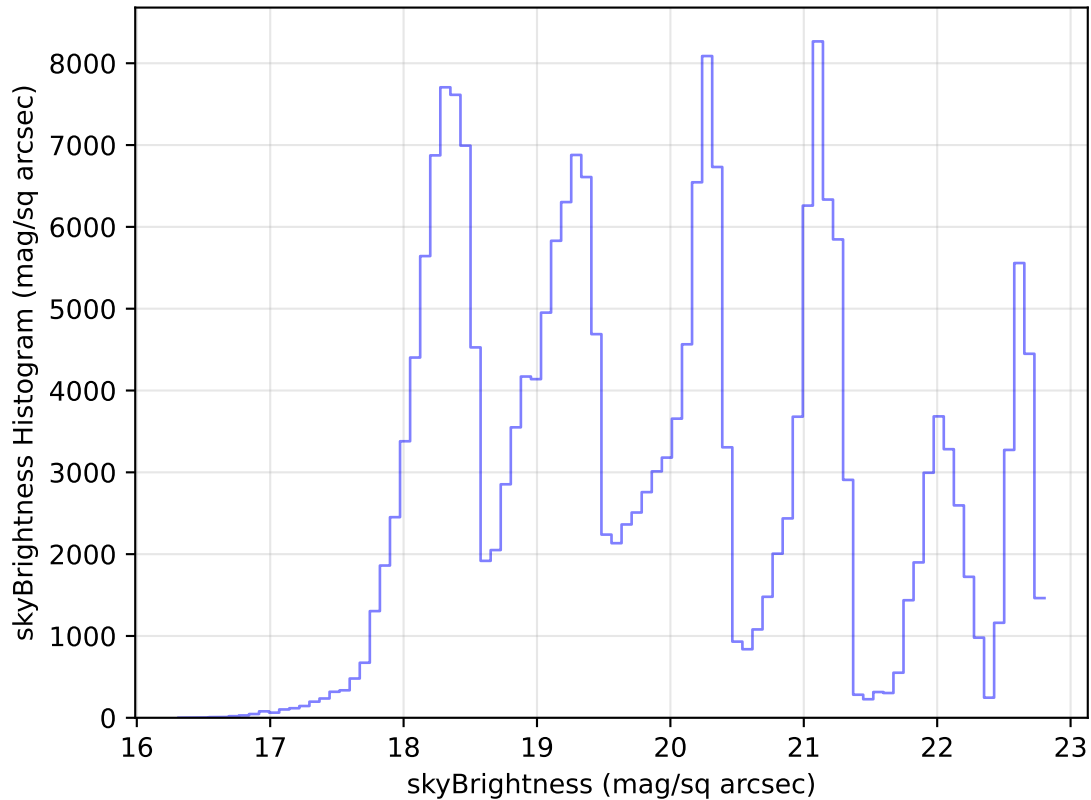
too_elab_r256_d3_ugrizy_v3.4_10yrs Yr 1 all bands: skyBrightness Histogram
