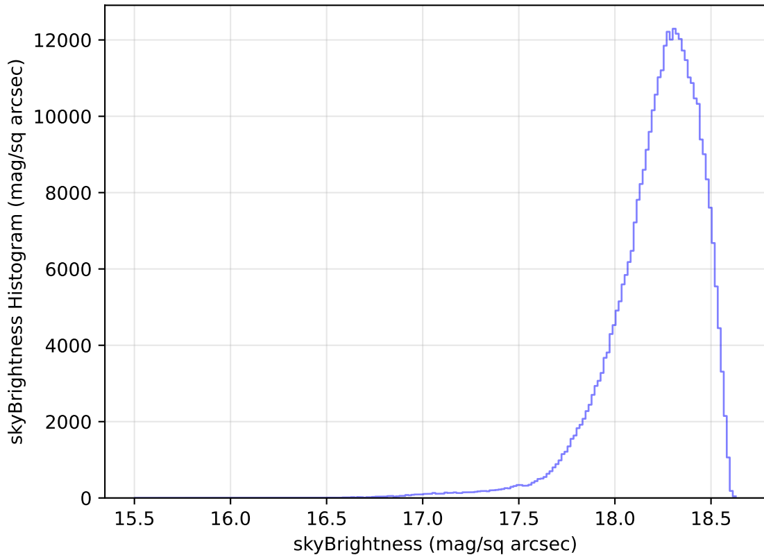
too_elab_r256_d3_ugrizy_v3.4_10yrs WFD y band: skyBrightness Histogram
