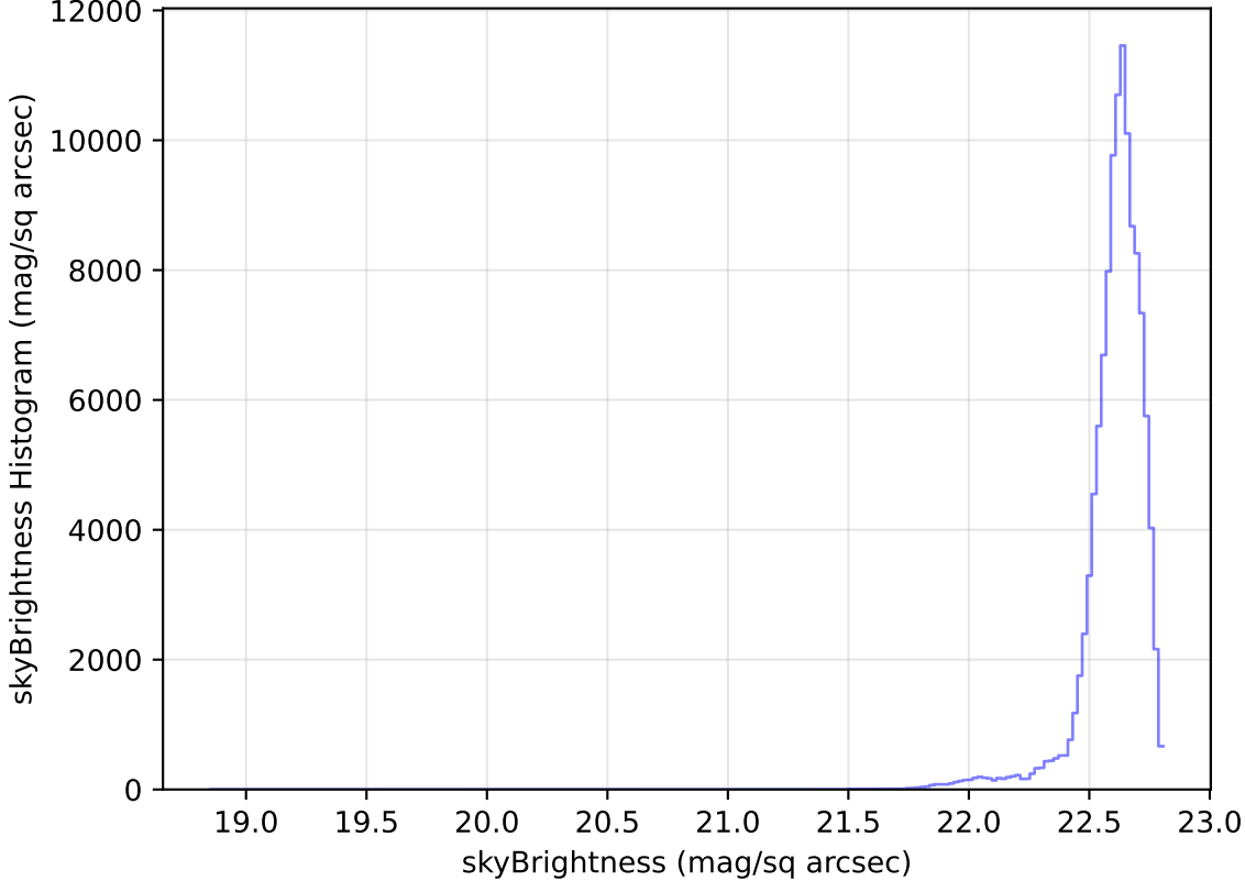
too_elab_r256_d3_ugrizy_v3.4_10yrs WFD u band: skyBrightness Histogram
