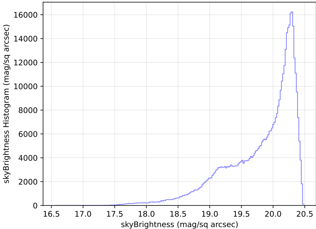
too_elab_r256_d3_ugrizy_v3.4_10yrs WFD i band: skyBrightness Histogram
