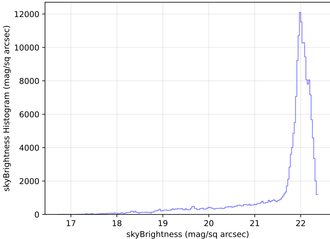
too_elab_r256_d3_ugrizy_v3.4_10yrs WFD g band: skyBrightness Histogram
