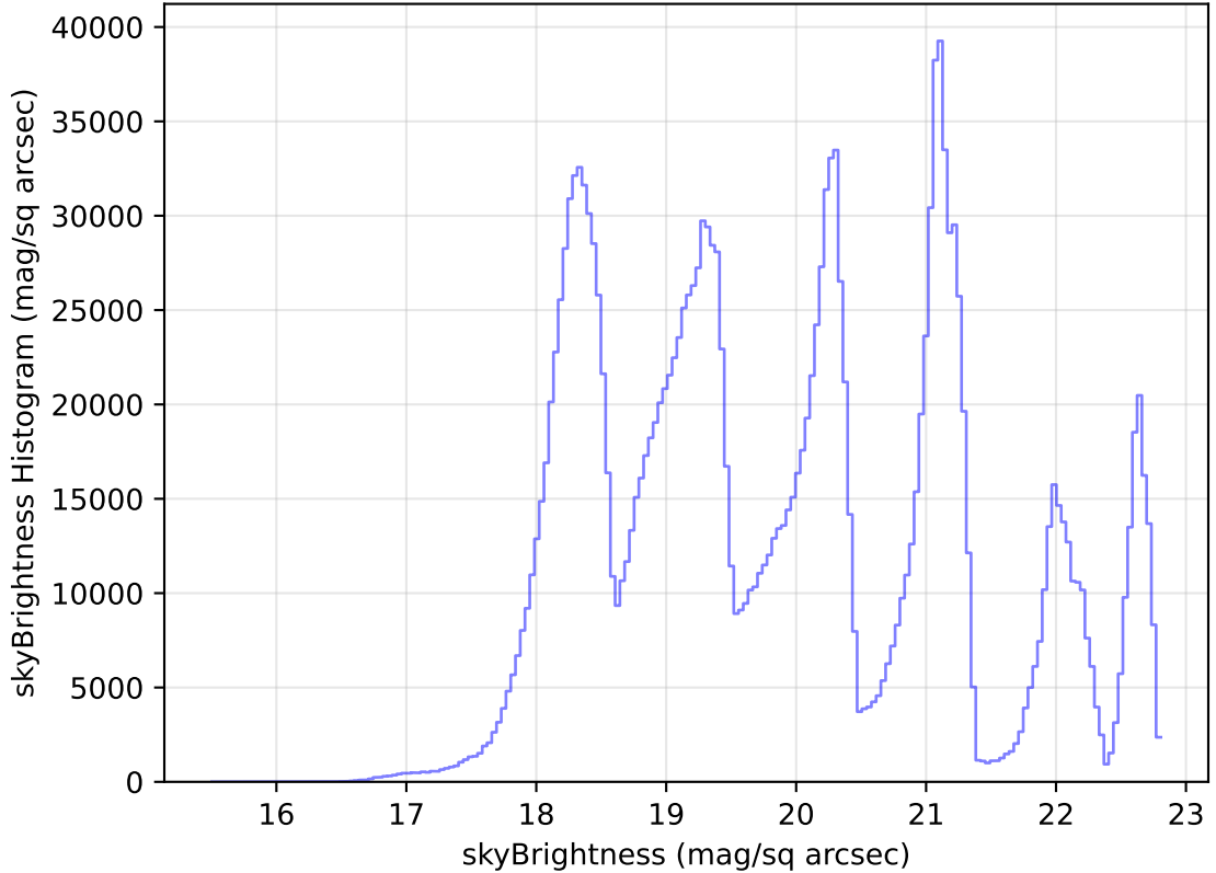
too_elab_r256_d3_ugrizy_v3.4_10yrs WFD all bands: skyBrightness Histogram
