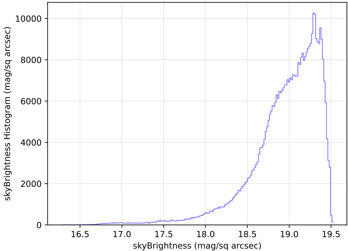
too_elab_r256_d3_ugrizy_v3.4_10yrs All sky z band: skyBrightness Histogram
