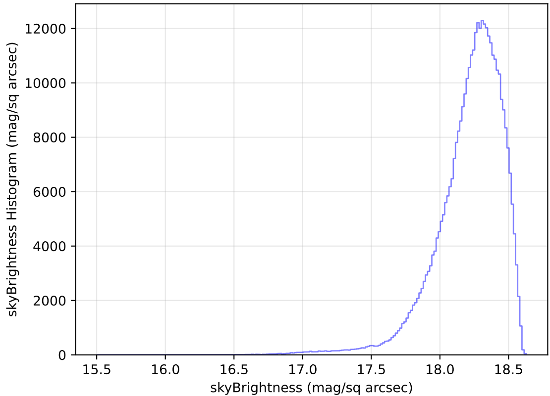
too_elab_r256_d3_ugrizy_v3.4_10yrs All sky y band: skyBrightness Histogram
