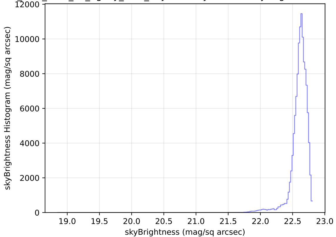
too_elab_r256_d3_ugrizy_v3.4_10yrs All sky u band: skyBrightness Histogram
