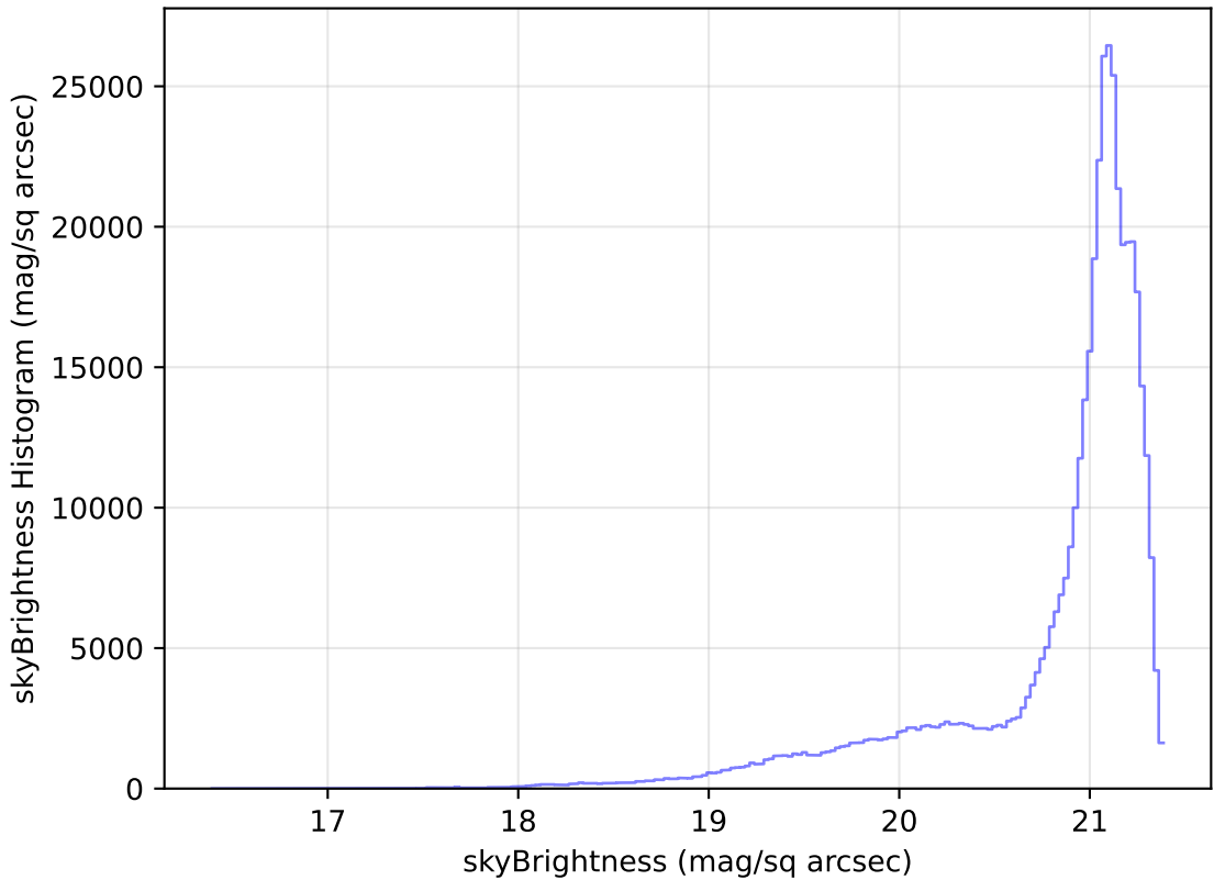
too_elab_r256_d3_ugrizy_v3.4_10yrs All sky r band: skyBrightness Histogram
