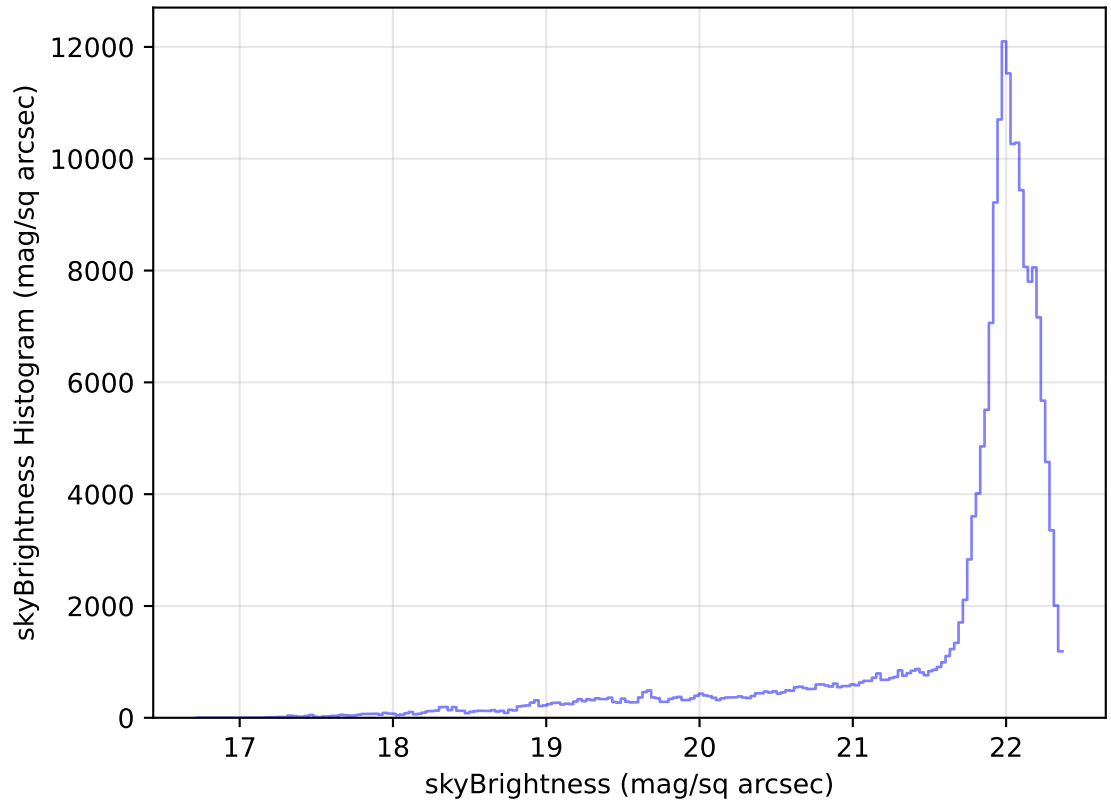
too_elab_r256_d3_ugrizy_v3.4_10yrs All sky g band: skyBrightness Histogram
