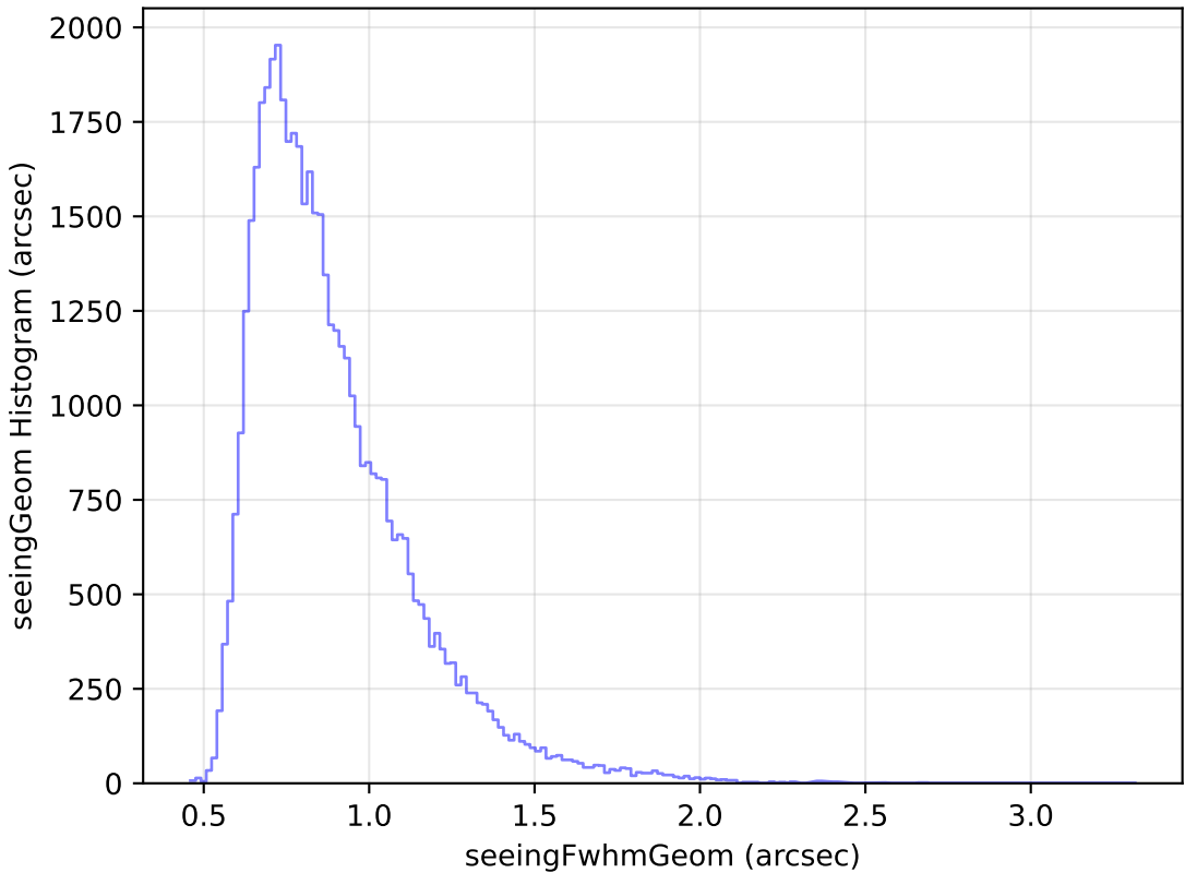
too_elab_r256_d3_ugrizy_v3.4_10yrs Yr 1 r band: seeingGeom Histogram
