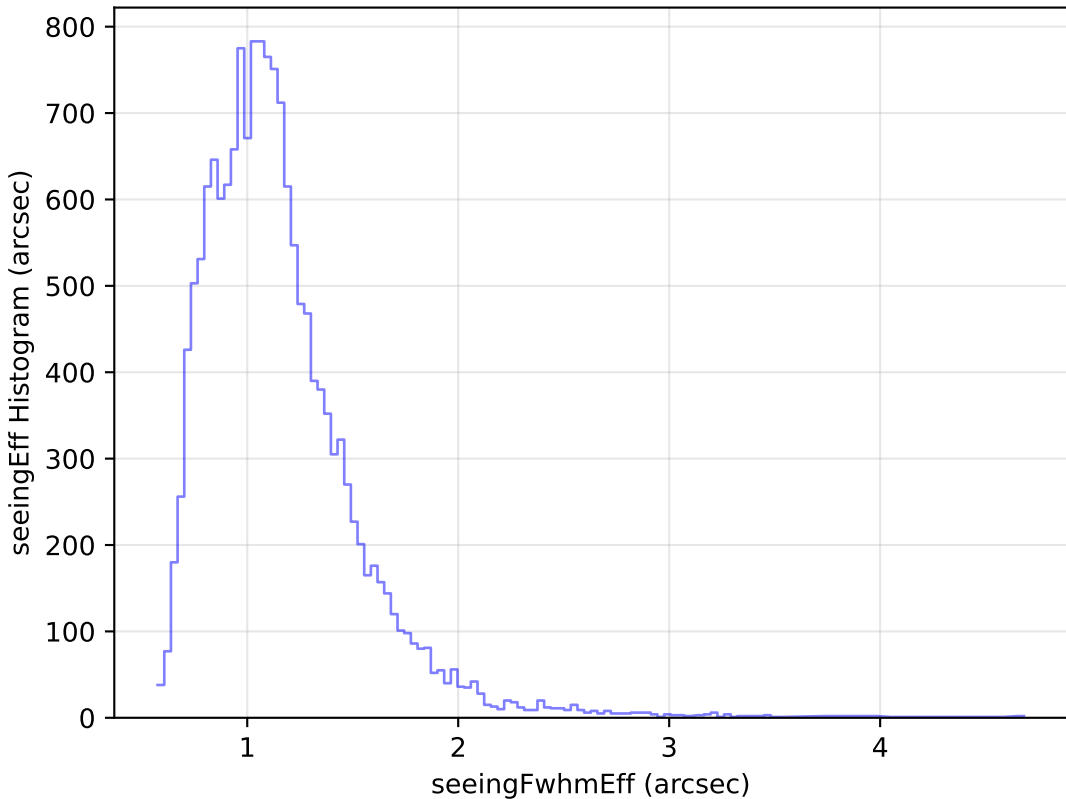
too_elab_r256_d3_ugrizy_v3.4_10yrs Yr 1 u band: seeingEff Histogram
