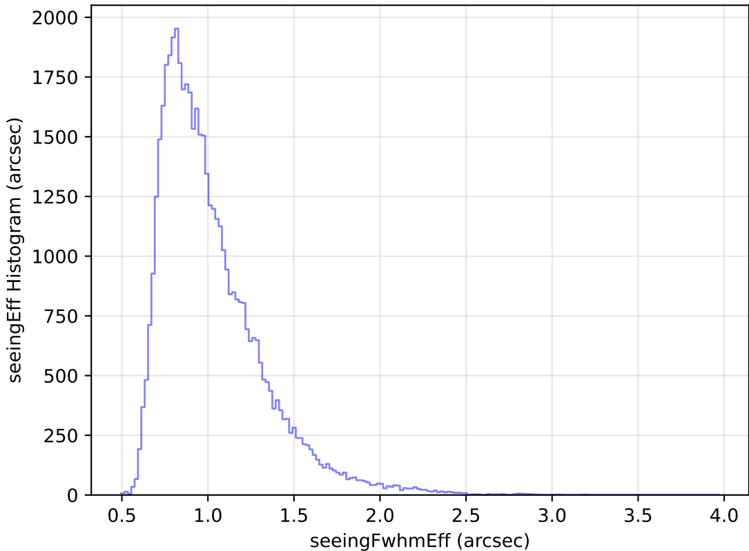
too_elab_r256_d3_ugrizy_v3.4_10yrs Yr 1 r band: seeingEff Histogram
