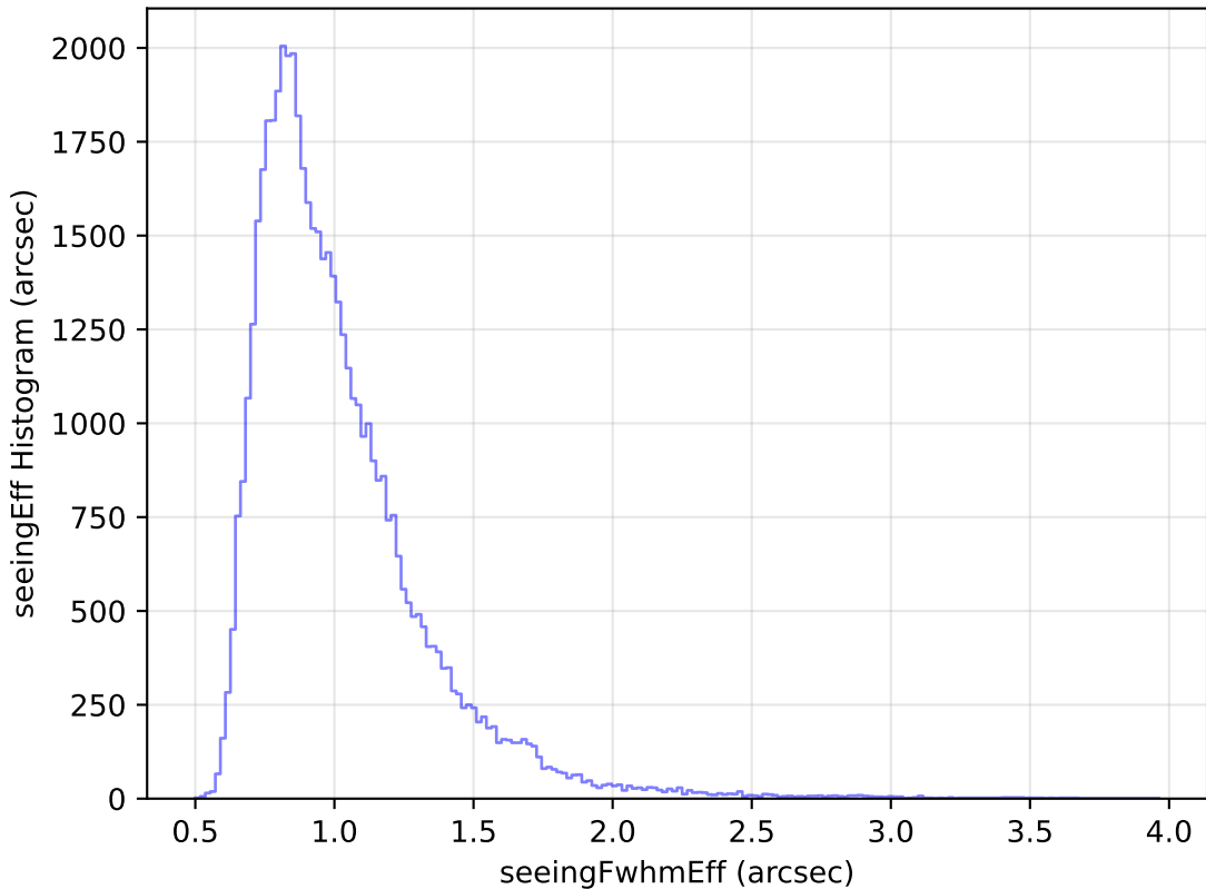
too_elab_r256_d3_ugrizy_v3.4_10yrs Yr 1 i band: seeingEff Histogram
